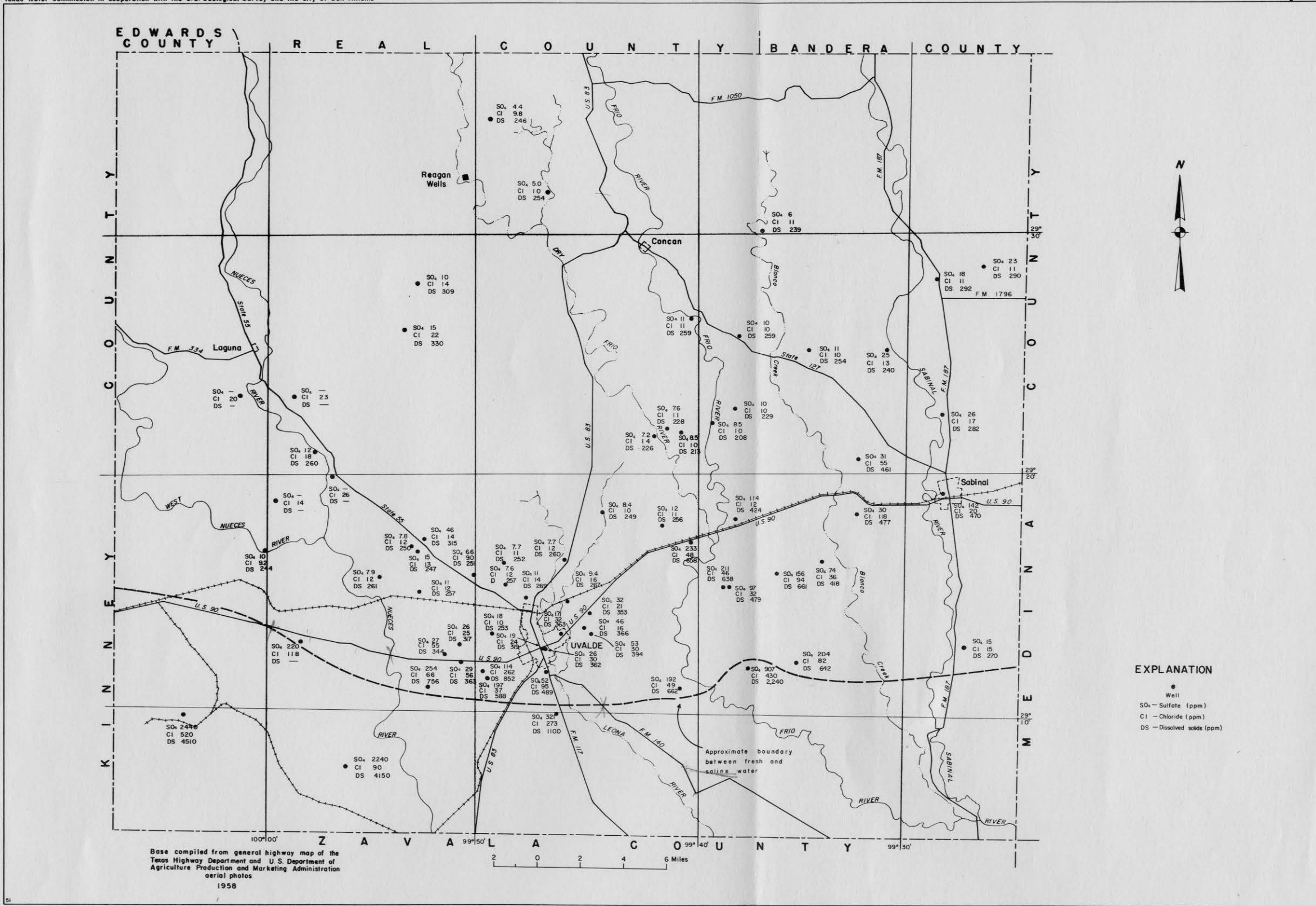
FIGURE 11.-Dissolved-solids, sulfate, and chloride concentrations in water from the Edwards and associated limestones, Uvalde County
