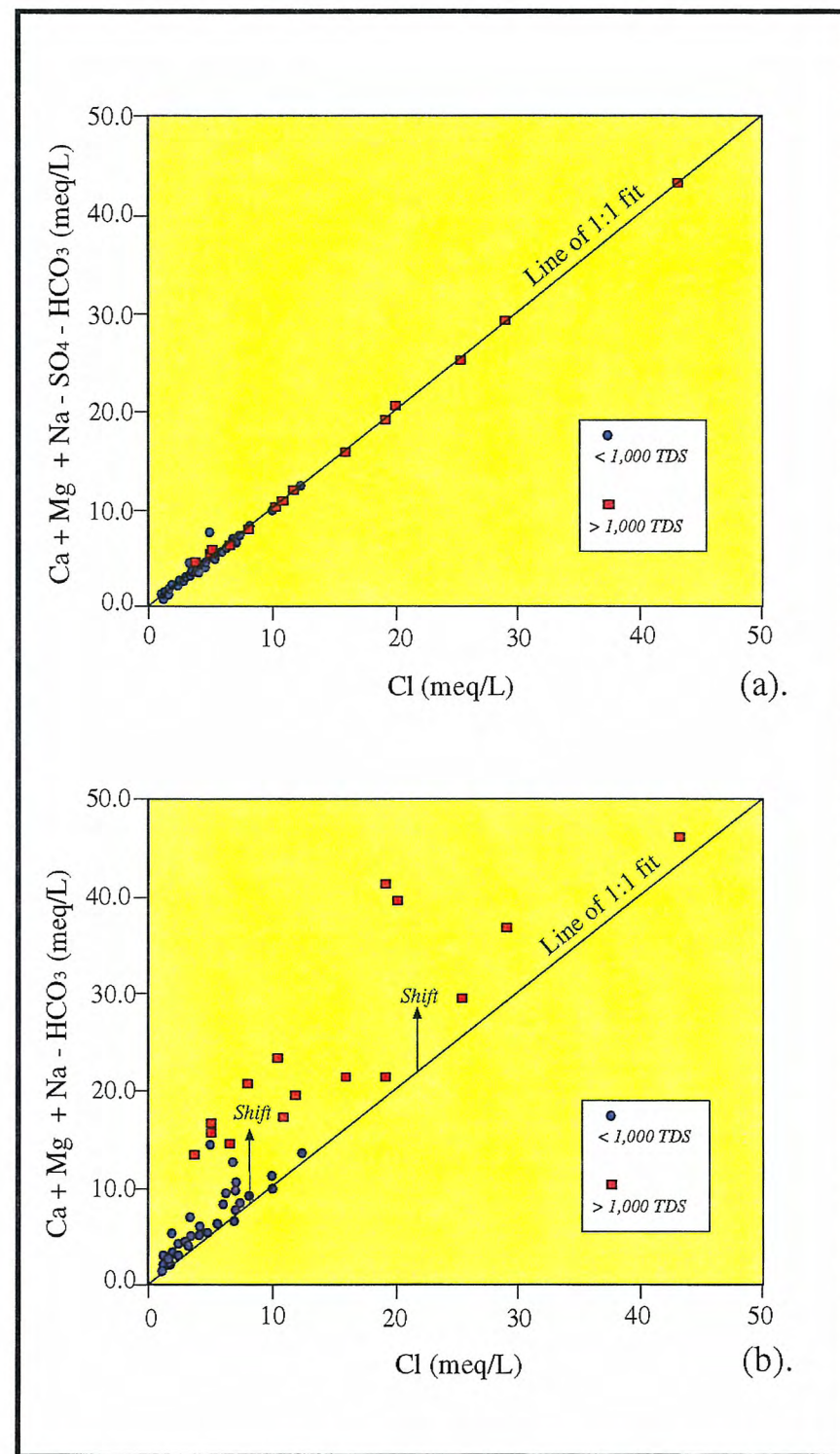
Figure 3.23. Upper figure (a); a plot of (\text{Ca} + \text{Mg} + \text{Na} - \text{SO}_4 - \text{HCO}_3) vs \text{Cl} in group 3 and group 4 ground waters gives an excellent 1:1 fit. Lower figure (b); the shift caused by removing (-\text{SO}_4) from the term (\text{Ca} + \text{Mg} + \text{Na} - \text{SO}_4 - \text{HCO}_3) gives the amount of mass due to dissolution of gypsum (source of data, Texas Water Development Board; Comision Nacional Del Agua; Instituto Nacional de Estadistica, Geografia e Informatica).
