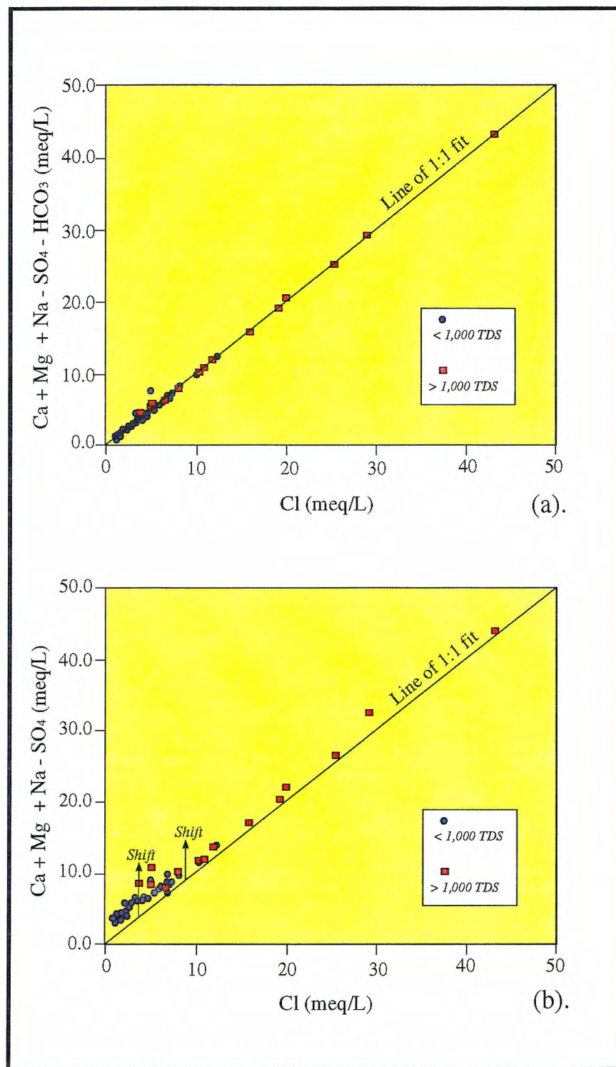
Figure 3.22. Upper figure (a); a plot of (\text{Ca} + \text{Mg} + \text{Na} - \text{SO}_4 - \text{HCO}_3) vs \text{Cl} in group 3 and group 4 ground waters gives an excellent 1:1 fit. Lower figure (b); the shift caused by removing (-\text{HCO}_3) from the term (\text{Ca} + \text{Mg} + \text{Na} - \text{SO}_4 - \text{HCO}_3) gives the amount of mass due to dissolution of calcite (source of data, Texas Water Development Board; Comision Nacional Del Agua; Instituto Nacional de Estadistica, Geografia e Informatica).
