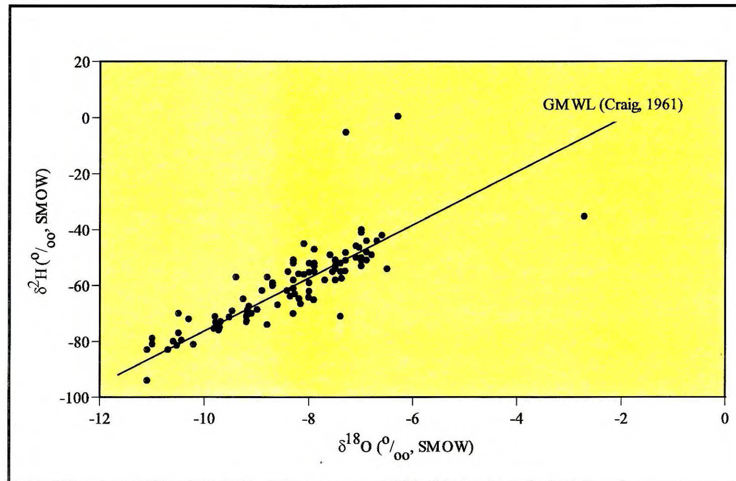
Figure 6.12. Plot of \delta^2\text{H} vs \delta^{18}\text{O} (source of data, Kreitler and others, 1986).
