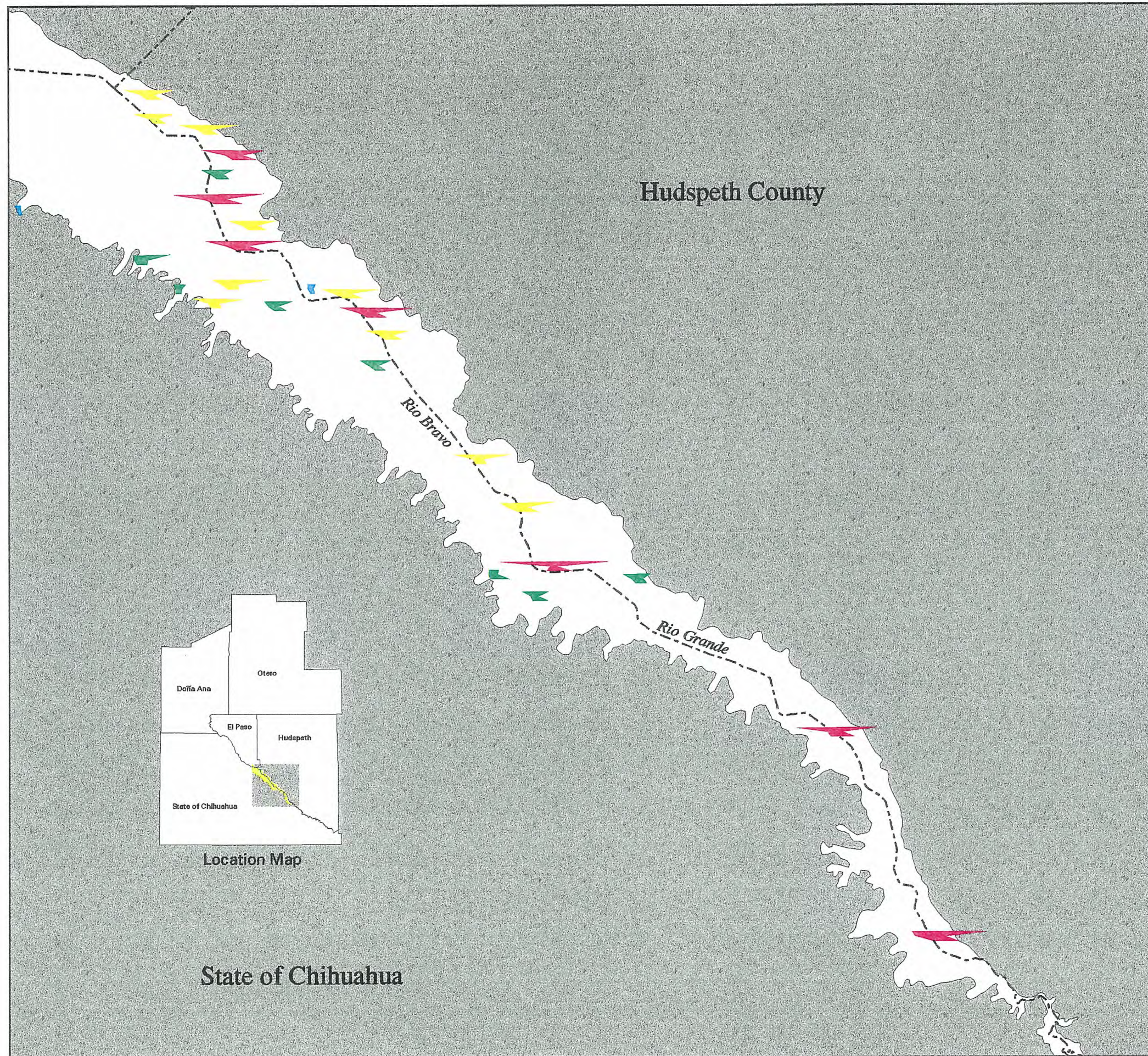
Figure 5.10. Stiff plots show Na-SQ-Cl ground waters with salinities usually greater than 3,000 mg/L in the Rio Grande aquifer below the El Paso/Hudspeth County line (source of data, Texas Water Development Board; Comision Nacional del Agua).
