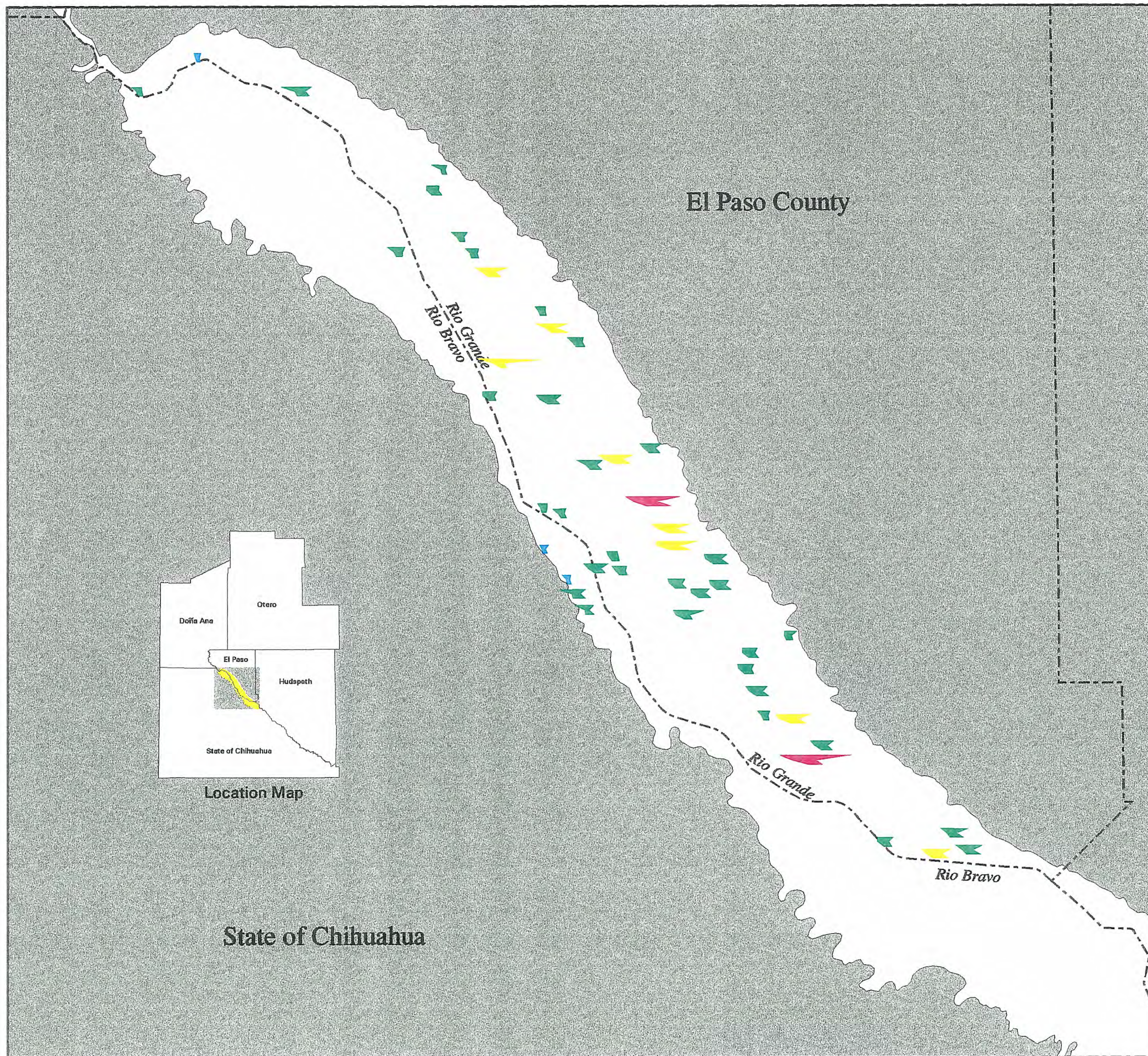
Figure 5.9. Stiff plots show Na-SO 4 ground waters with salinities usually less than 3,000 mg/L in the Rio Grande aquifer above the El Paso/Hudspeth County line (source of data, Texas Water Development Board; Comision Nacional del Agua).
