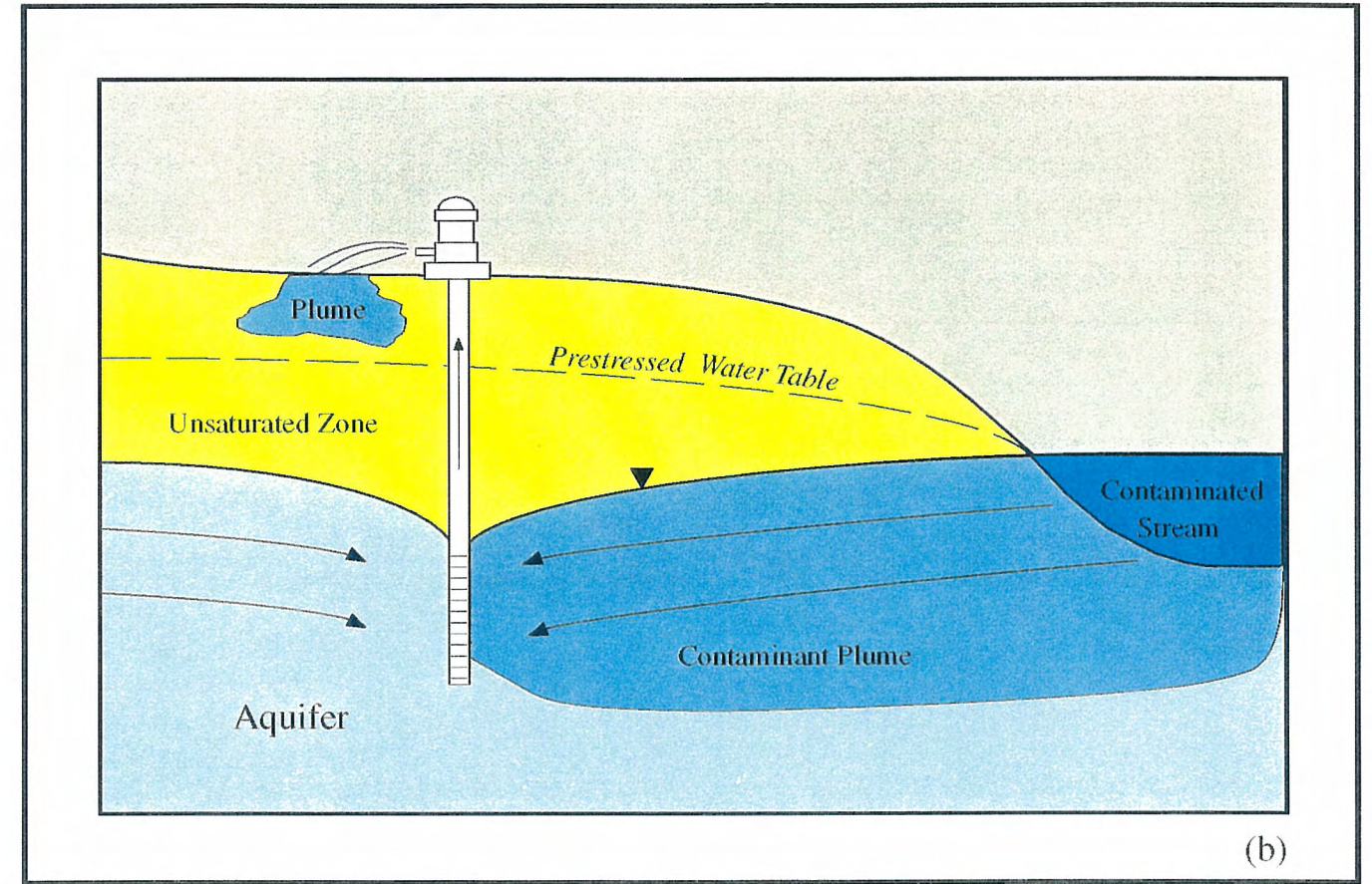
Figure 5.23b. Diagram illustrating contamination of an alluvial aquifer from a contaminated stream. Induced infiltration of contaminated surface water may contaminate the aquifer.
