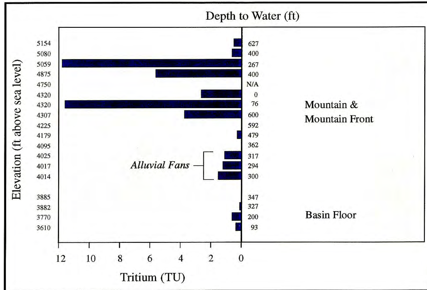
Figure 4.6a. Tritium activities (TU) in highland (mountain and mountain front) and lowland (basin floor) areas of the southeastern Hueco aquifer indicate that precipitation recharge occurs primarily within the upper mountains and plateaus (source of data, Fisher and Mullican, 1990).
