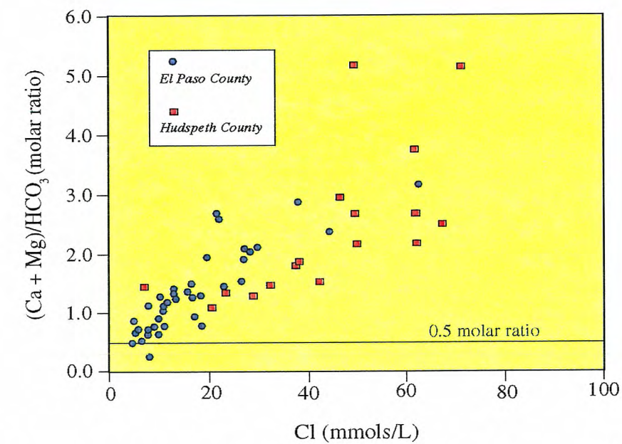
Figure 5.19. Scatter plot showing (Ca+Mg)/ \text{HCO}_3 molar ratios vs molar Cl for samples collected from the Rio Grande aquifer in El Paso and Hudspeth Counties. Points above the 0.5 ratio line indicate a source of calcium and/or magnesium other than dissolution of carbonate rock (source of data, Texas Water Development Board).
