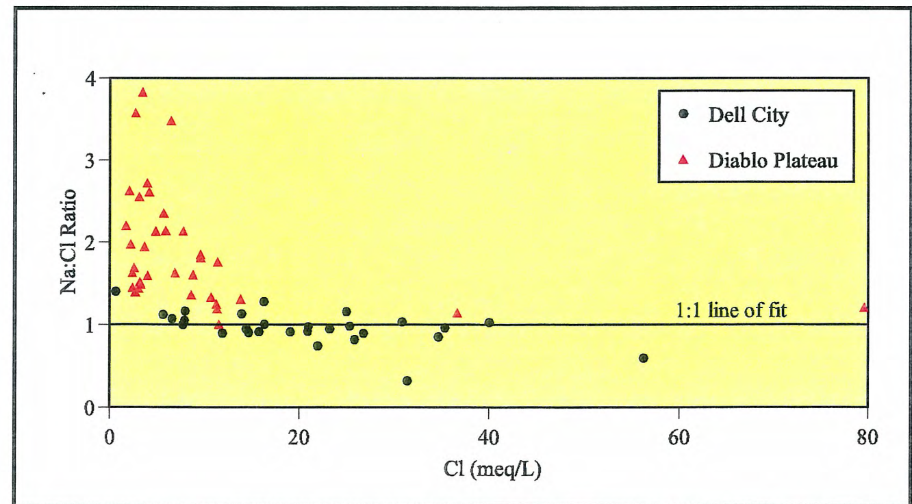
Figure 6.10. Plot of (Na/Cl) ratio vs Cl.
