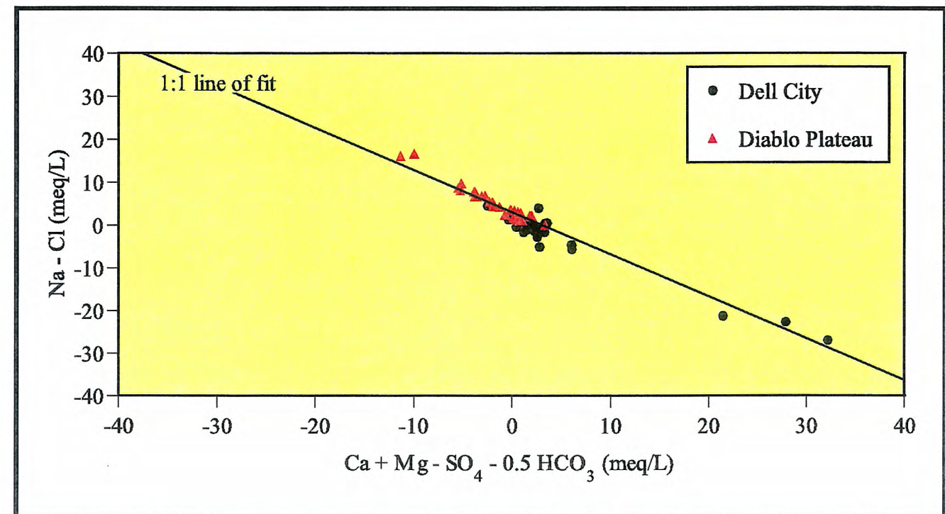
Figure 6.9. Plot of (Na - Cl) vs (Ca + Mg - SO 4 - 0.5HCO 3 ).
