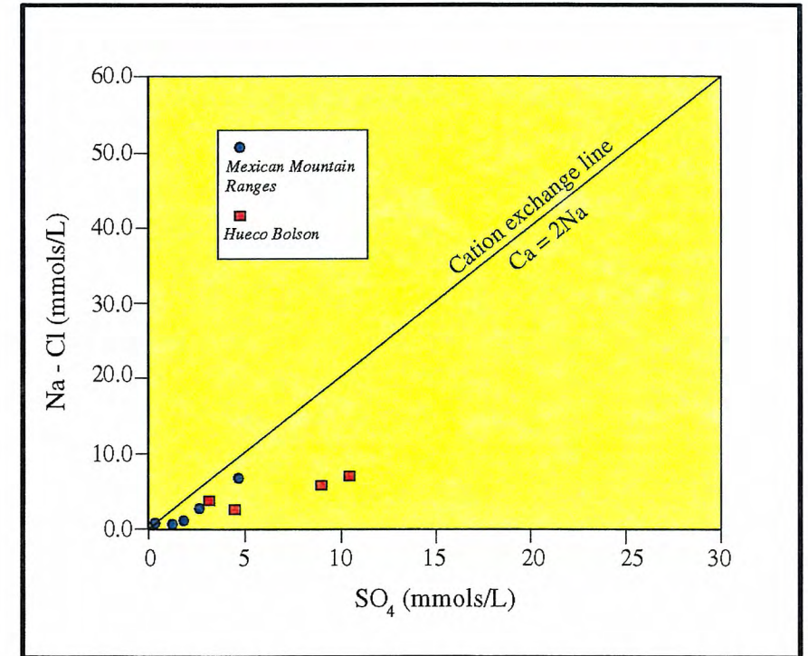
Figure 4.10b. Scatter plot showing (Na - Cl) molar quantity vs molar SO_4 for samples collected from bedrock strata and bolson strata, Mexico (source of data, Comision Nacional Del Agua; Instituto Nacional de Estadistica, Geografia e Informatica).
