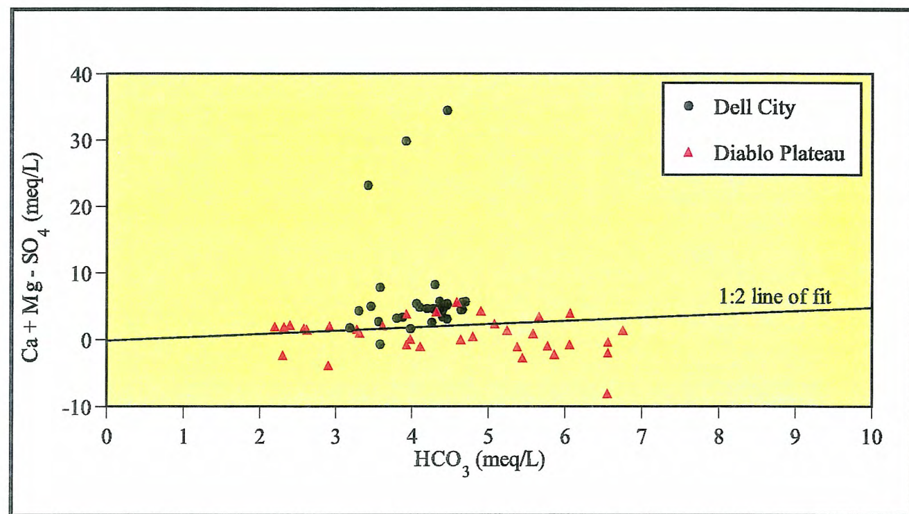
Figure 6.8. Plot of (Ca + Mg - SO 4 ) vs HCO 3 .
