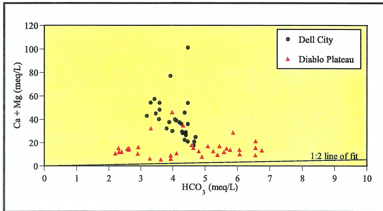
Figure 6.7. Plot of (Ca + Mg) vs HCO 3 .
