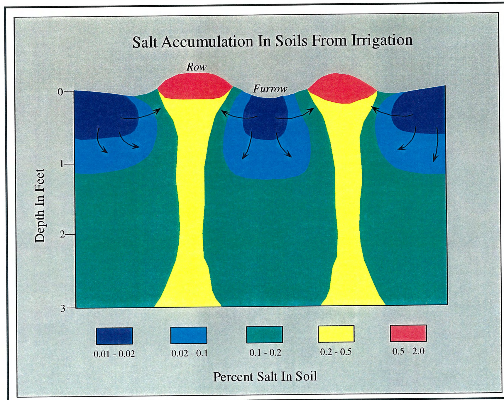
Figure 5.11. Diagram showing how dissolved salts in irrigation water become concentrated in irrigated soils due to high evapotranspiration rates (modified from Longnecker and Lyerly, 1959).
