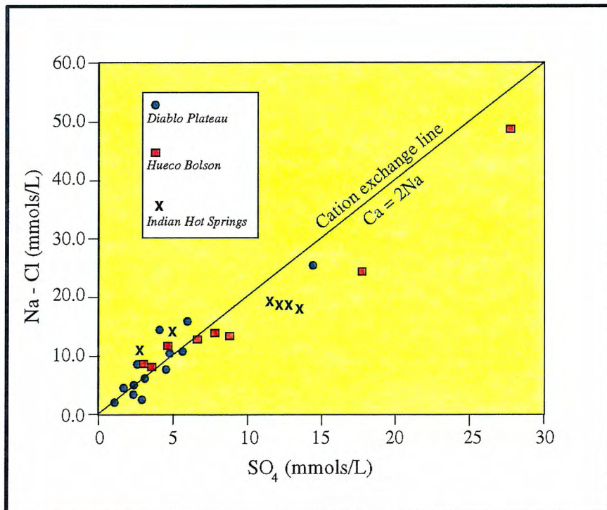
Figure 4.10a. Scatter plot showing (Na - Cl) molar quantity vs molar SO_4 for samples collected from bedrock strata, bolson strata, and Indian Hot Springs, U.S. (source of data, Fisher and Mullican, 1990; Darling and others, 1994; Texas Water Development Board).
