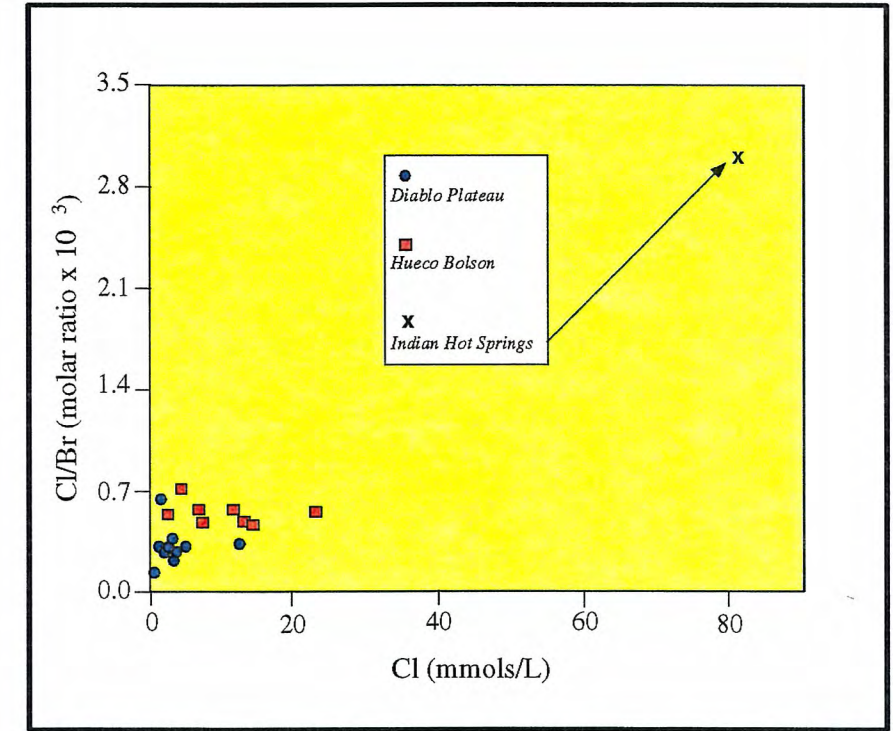
Figure 4.9. Scatter plot showing (Cl/Br) molar ratios vs molar Cl for samples collected from bedrock strata, bolson strata, and Indian Hot Springs, U.S. (source of data, Fisher and Mullican, 1990; Darling and others, 1994; Texas Water Development Board).
