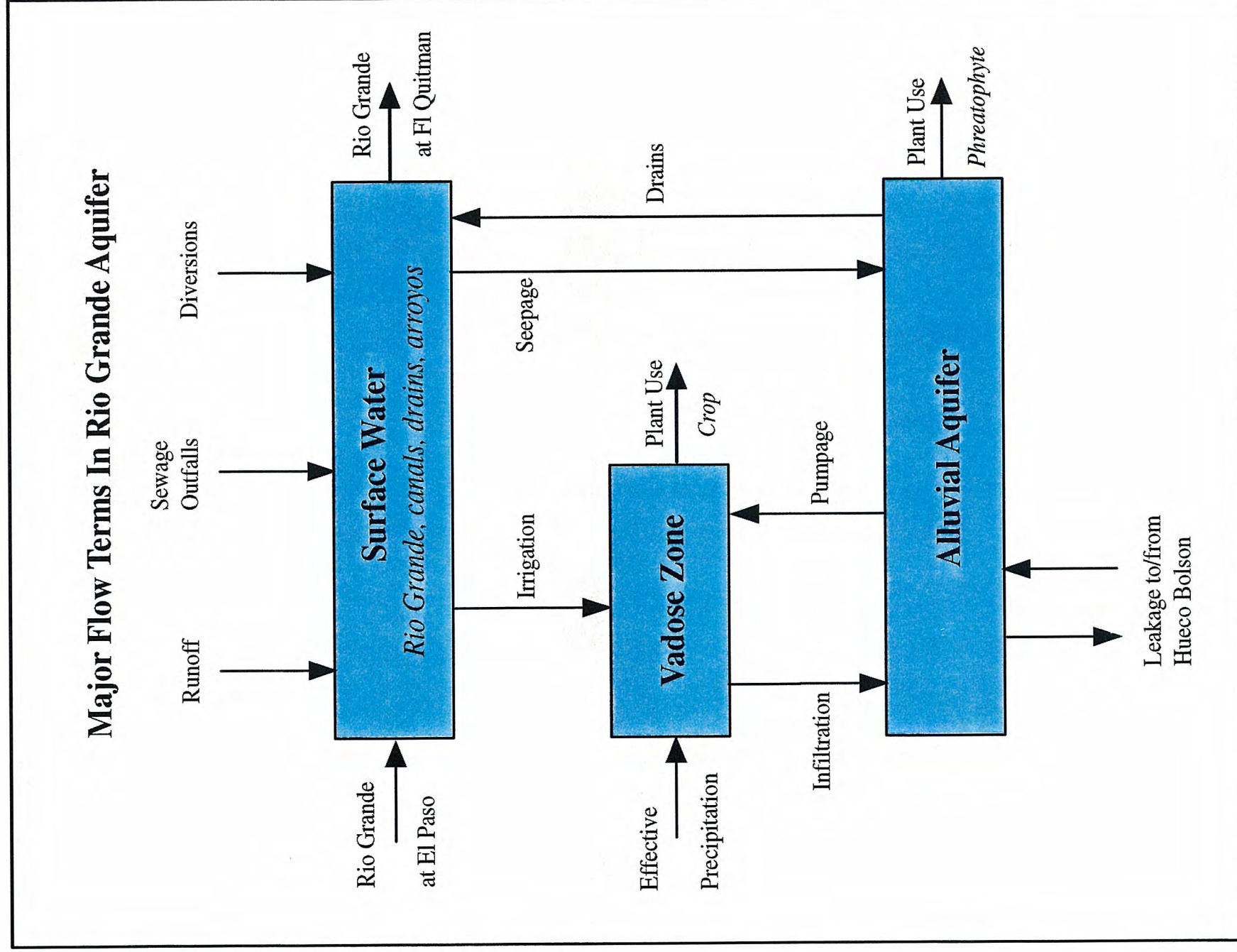
Figure 5.7. Major flow components in the Rio Grande aquifer.
