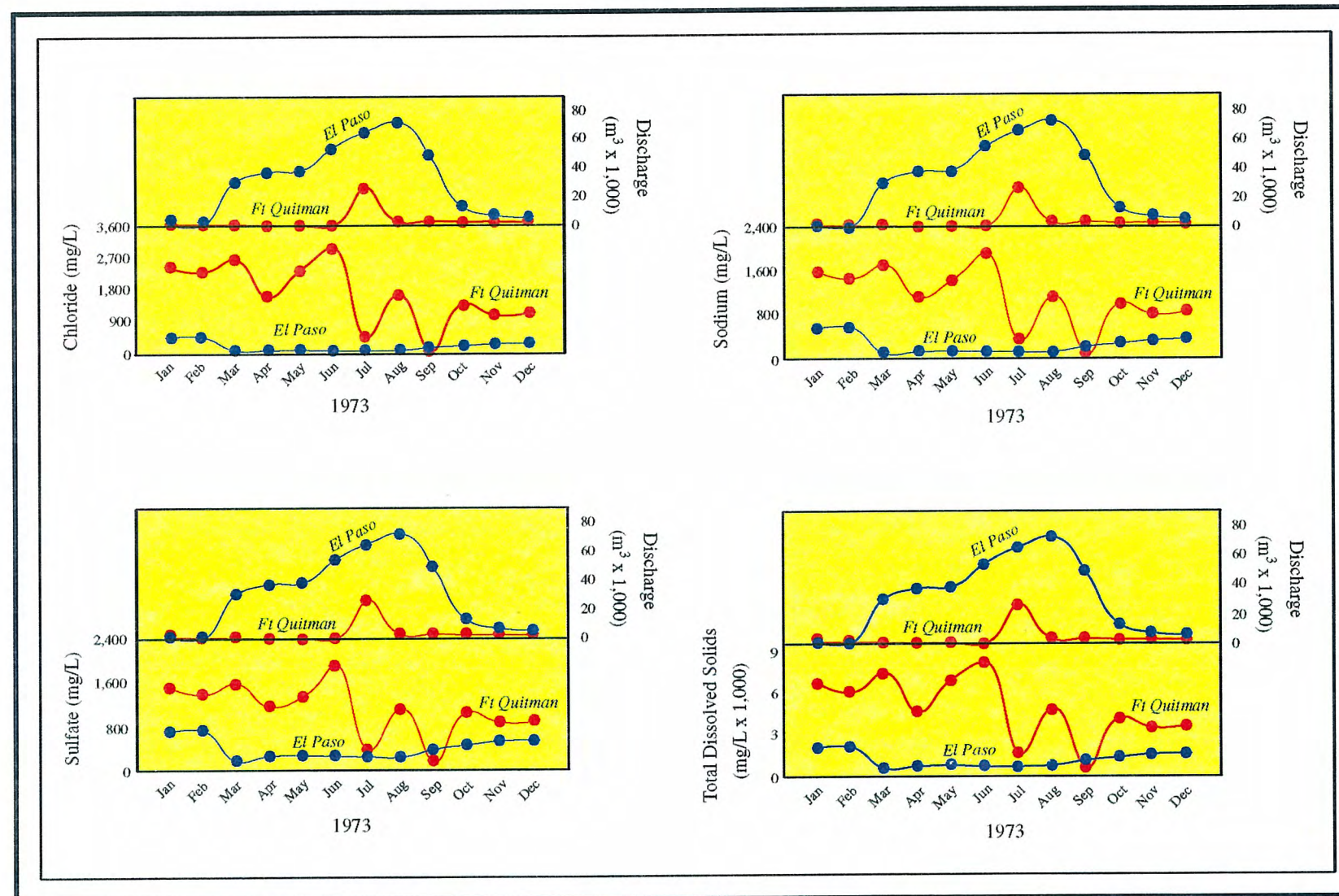
Figure 5.12a. Diagram comparing water quality and streamflow discharge for the Rio Grande at El Paso and Ft Quitman, 1973. Spatial changes in Cl , SO_4 , Na , and TDS for most months indicate appreciable decline in surface-water quality downstream of El Paso. Water quality improves when discharge is high as an artifact of dilution by large quantities of dilute reservoir water and by stagnation of saline baseflow as a result of high river stage (source of data, IBWC Water Bulletin series "Flow of the Rio Grande and Related Data").
