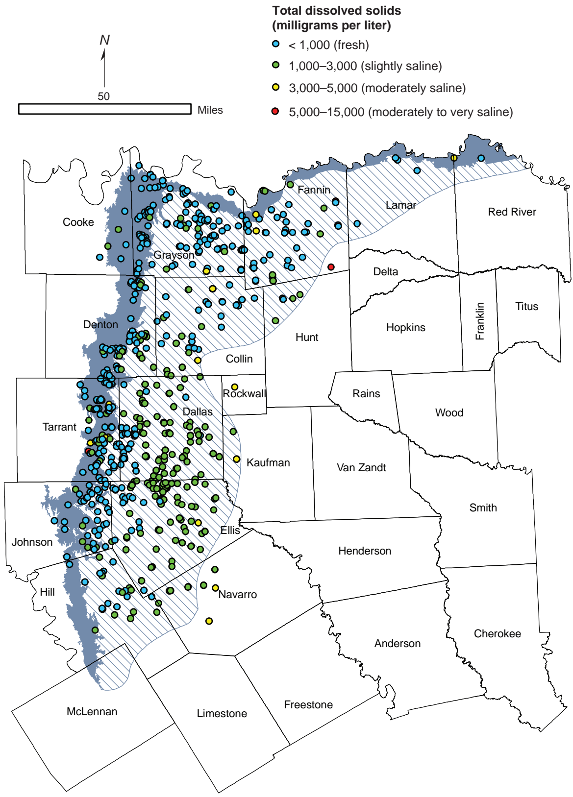
Total dissolved solids from Woodbine Aquifer wells (based on TWDB groundwater database).
