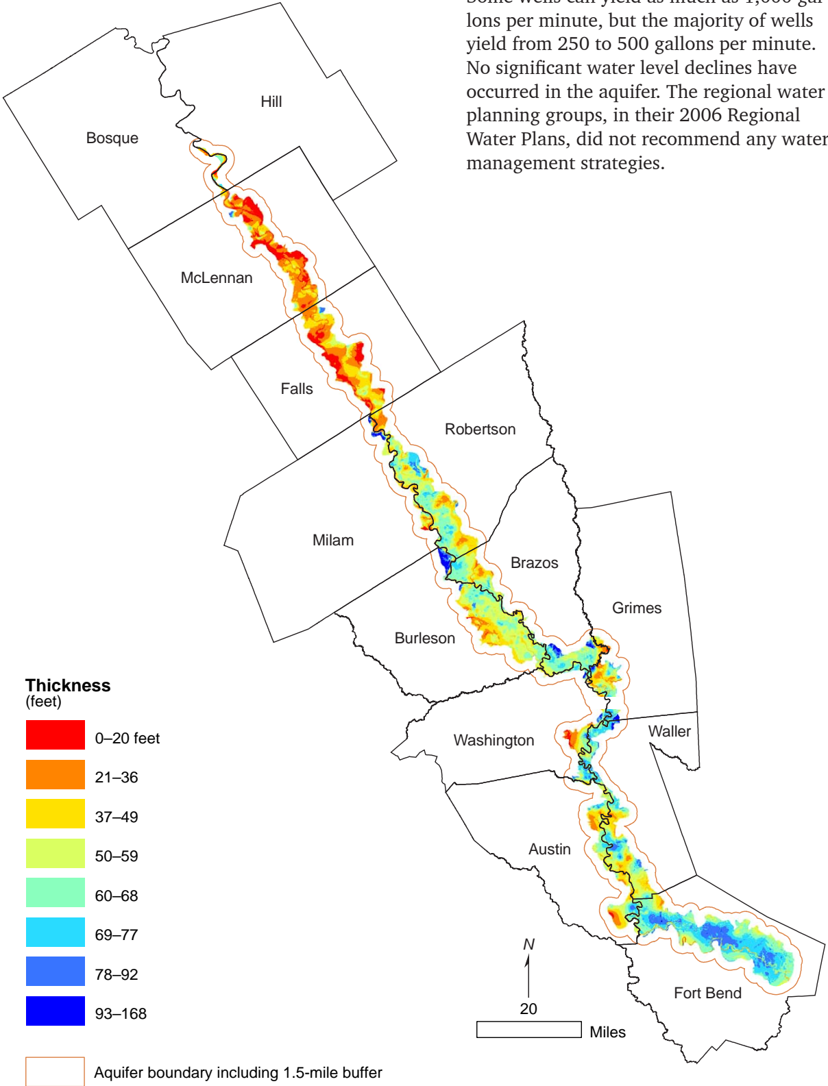
Thickness of the Brazos River Alluvium Aquifer, Bosque County to Fort Bend County, Texas (from Shah and others, 2007).
