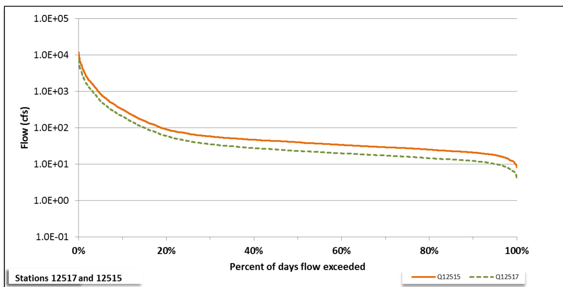
Figure 14. Flow duration curve for the Above Tidal (Station 12517) and Tidal (Station 12515) locations.
